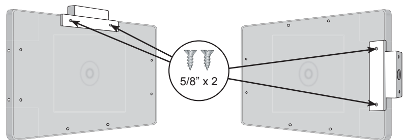
CEILING MOUNT
